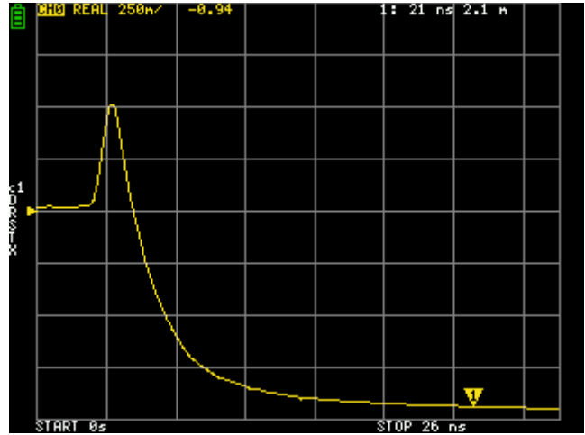
Inductive short
