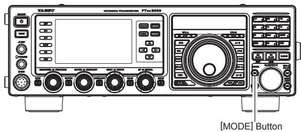
[MODE] Button
