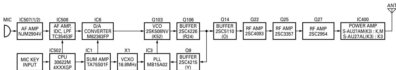
Fig. 8 Transmitter system
