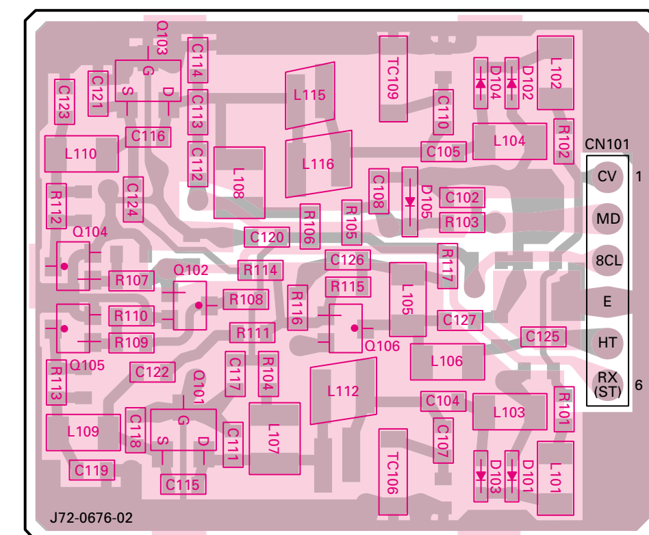
PLL/VCO (X58-4670-XX) -12 : K,M -14 : K3 Foil side view
