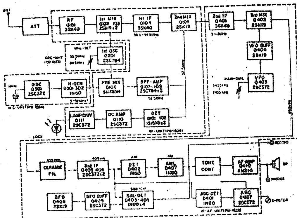
Fig.4 BLOCK DIAGRAM
