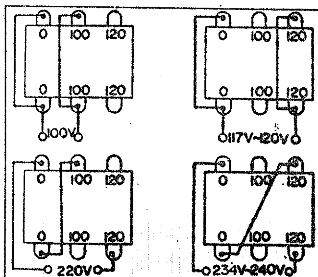
Fig.1 Transformer Primary Wiring
