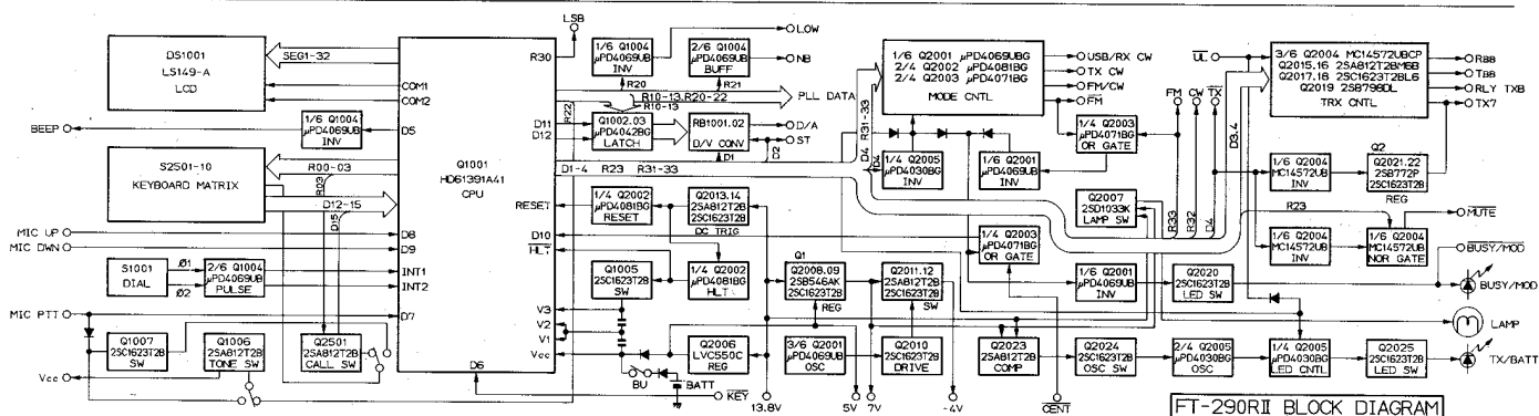
FT-290RII BLOCK DIAGRAM
