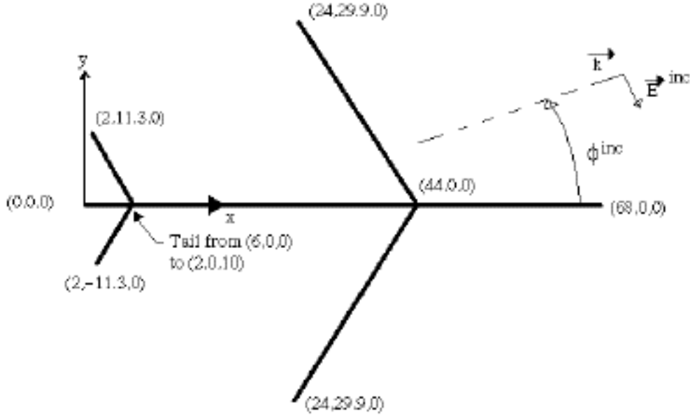
Figure 19. Stick model of aircraft.
