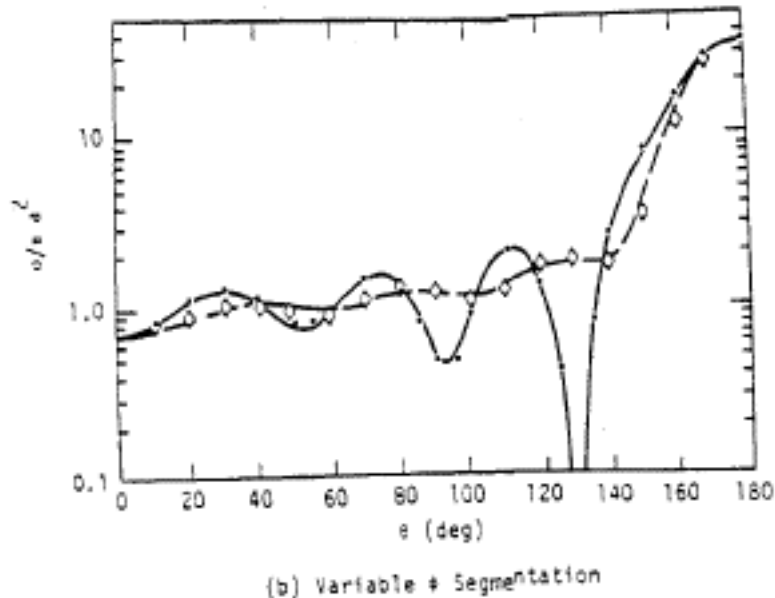
Figure 4. Bistatic RCS of a Sphere with ka = 5.3 (continuation).
