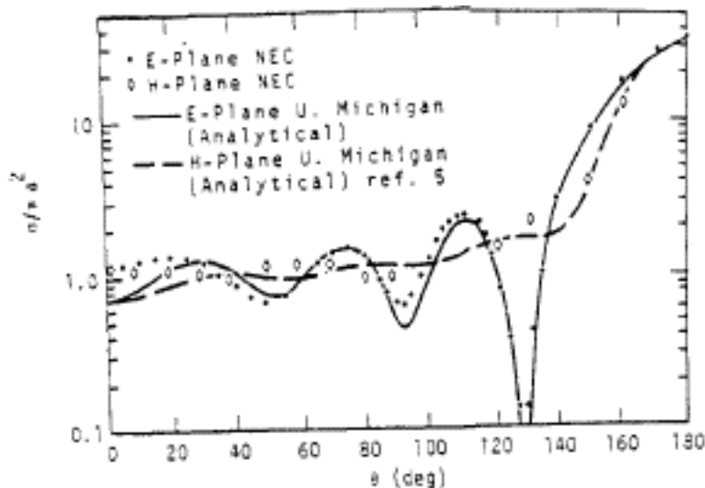
(a) Uniform Segmentation
