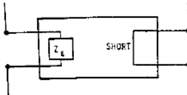
Figure 17. Segment Loaded by Means of a 2-Port Network.
