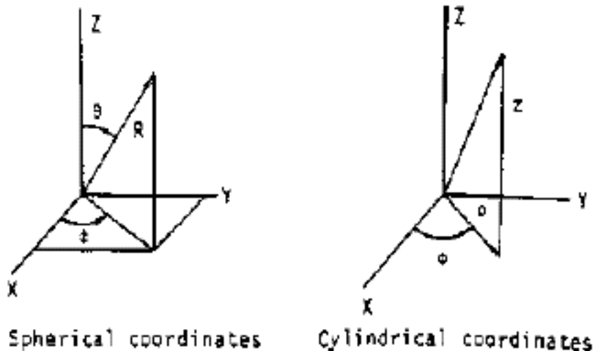
Figure 18. Coordinates for Radiated Field.
