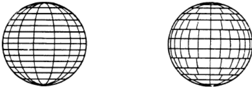
Uniform Segmentation
