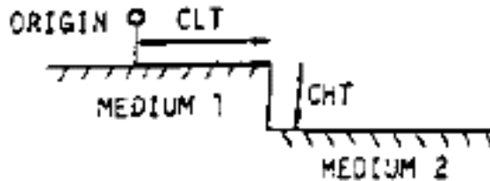
Figure 16. Parameters for a second Ground Medium
