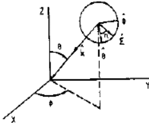
Figure 14. Specification of Incident Wave.
