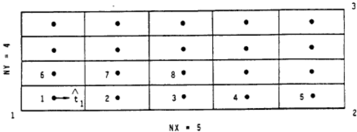
Figure 6. Rectangular Surface Covered by Multiple Patches.
