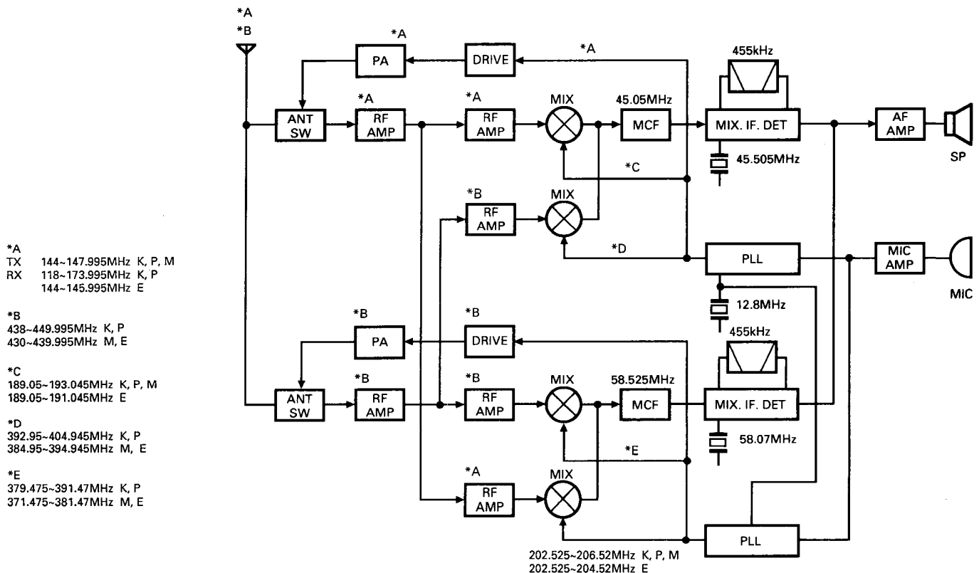
Fig.1 Frequency configuration
