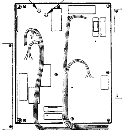
MAIN unit
