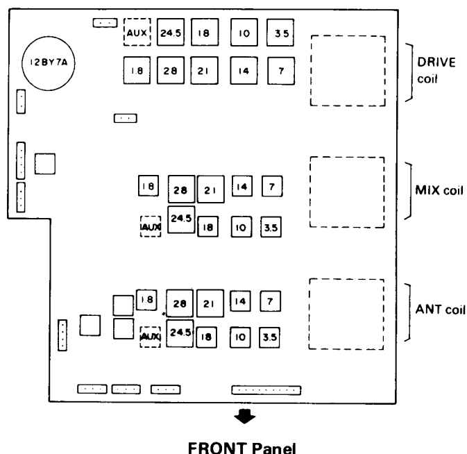
Fig. 6-1 Coil Pack Locations
