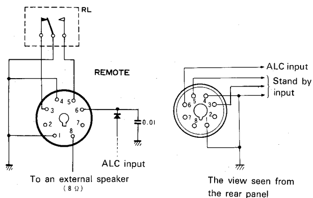
Fig. 32 REMOTE Connector
