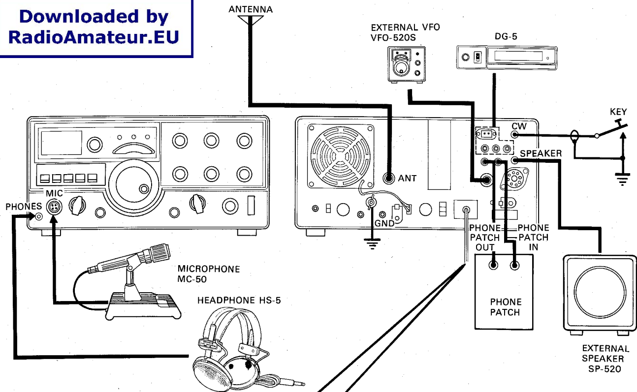
Fig. 1 (A) Cabling
