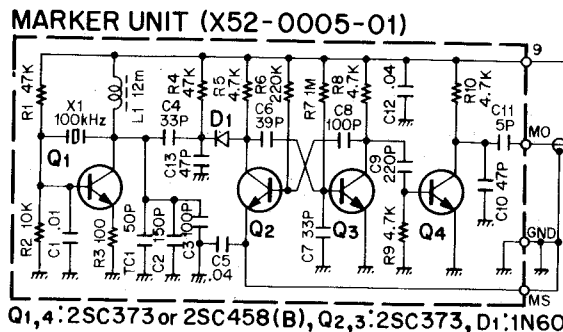
Fig. 21 Marker Board
