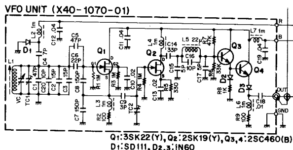
Fig. 20 VFO Board
