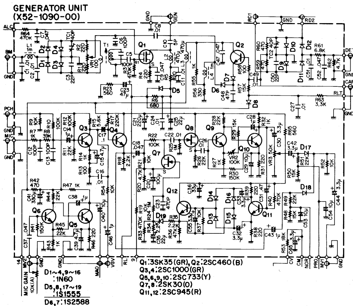
Fig. 15 Generator Board
