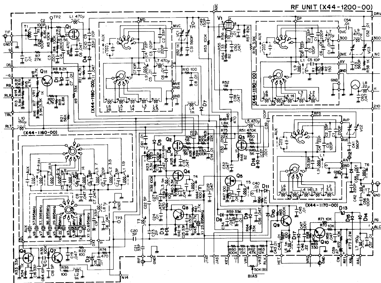
Fig. 16 RF Board
