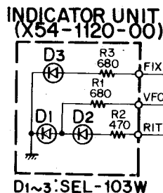
Fig. 26 Indicator Board
