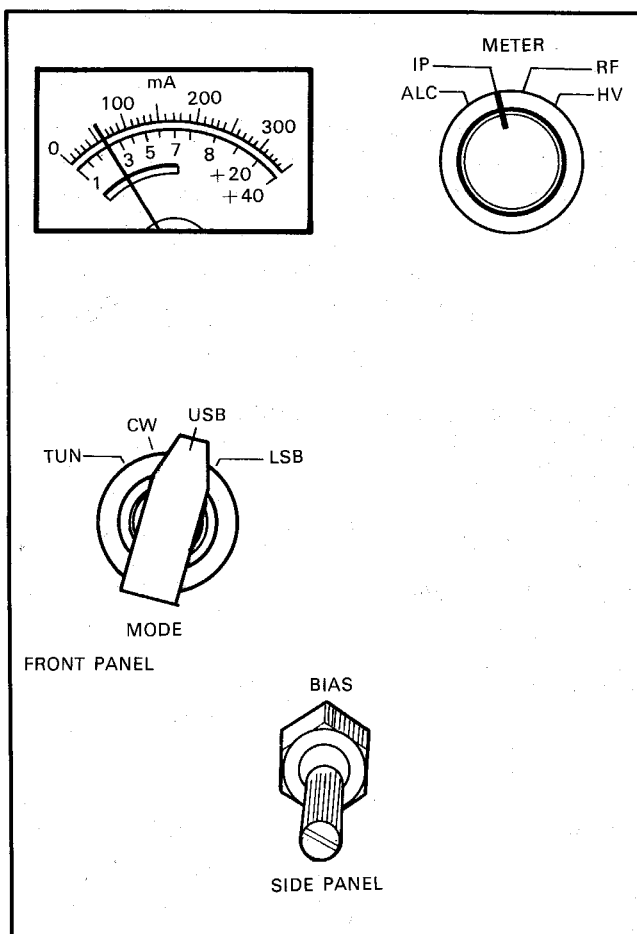
Fig. 10 Adjustment of the Plate Idling Current
