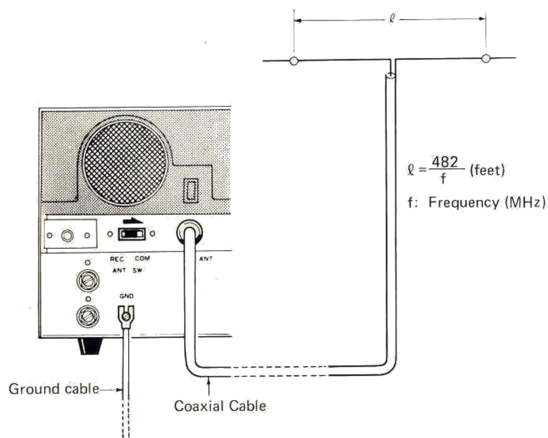
Fig. 6 Antenna Connections
