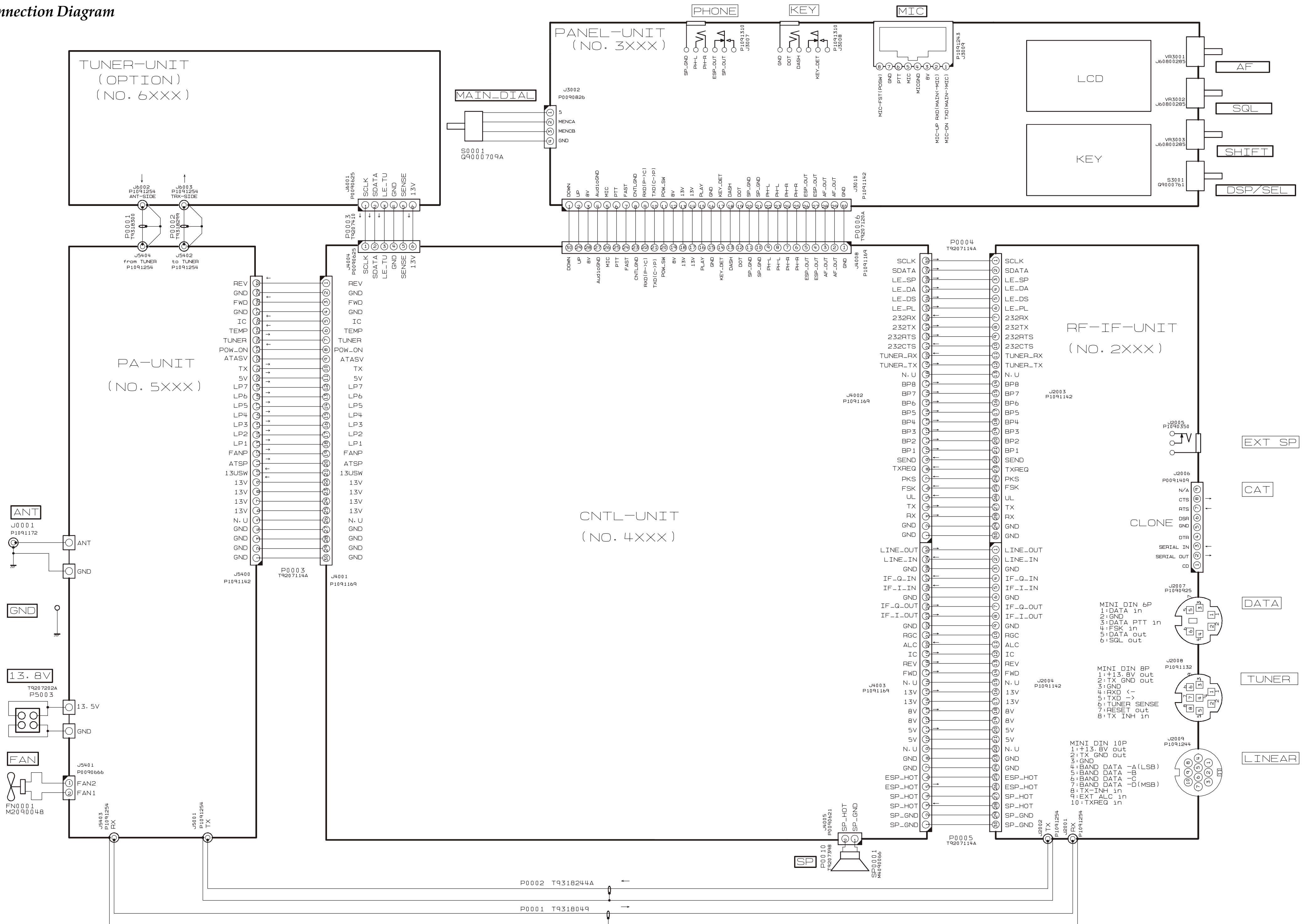
CONNECTION DIAGRAM-1
