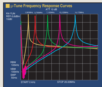
10 dB/Div • 2 MHz/Div
