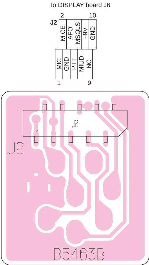
• BOTTOM VIEW (MIC BOARD)
