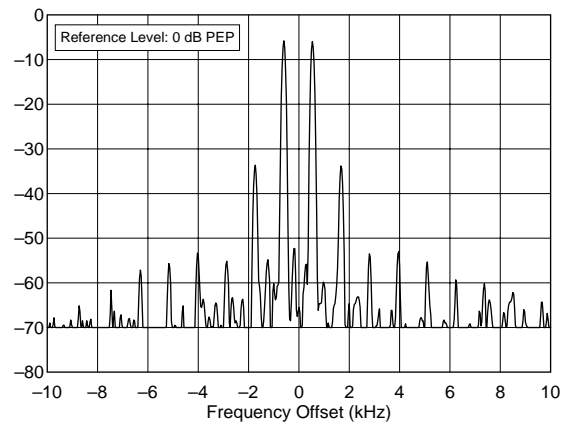
Kenwood TS-2000 s/n 20800064 10.120 MHz, Transmit IMD, 100 W F:\SHARED\PROD_REV\TESTS\TS2000\TS200130.TXT
