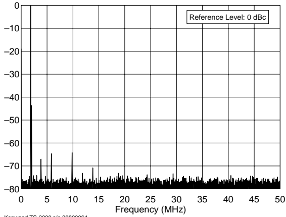
Kenwood TS-2000 s/n 20800064 1.8 MHz Band, Spectral Purity, 100 W F:\SHARED\PROD_REVTESTS\TS2000\TS200SLO.TXT
