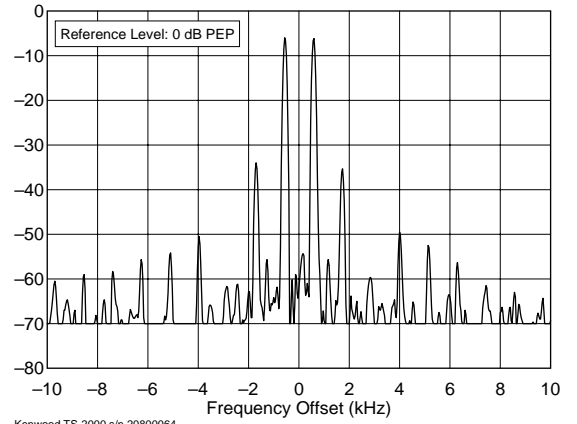
Kenwood TS-2000 s/n 20800064 7.250 MHz, Transmit IMD, 100 W F:\SHARED\PROD_REV\TESTS\TS2000\TS200140.TXT
