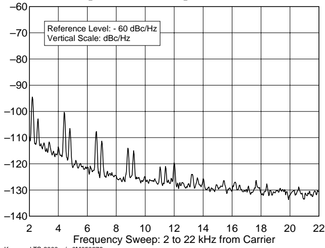
Kenwood TS-2000, s/n 0M050276 3.520 MHz, Phase Noise, 100 W F:\SHARED\PROD_REV\TESTS\TS2000\TS200P80.TXT
