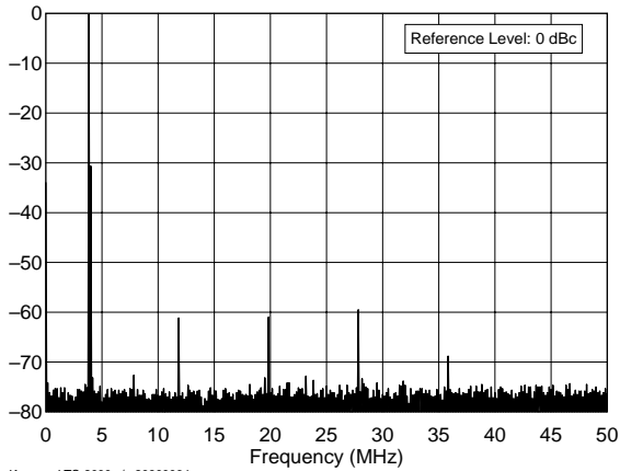
Kenwood TS-2000 s/n 20800064 3.5 MHz Band, Spectral Purity, 100 W F:\SHARED\PROD_REVTESTS\TS2000\TS200S80.TXT
