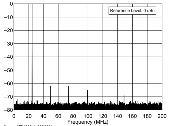
Kenwood TS-2000 s/n 20800064 24.9 MHz Band, Spectral Purity, 100 W F:\SHARED\PROD_REV\TESTS\TS2000\TS200S12.TXT
