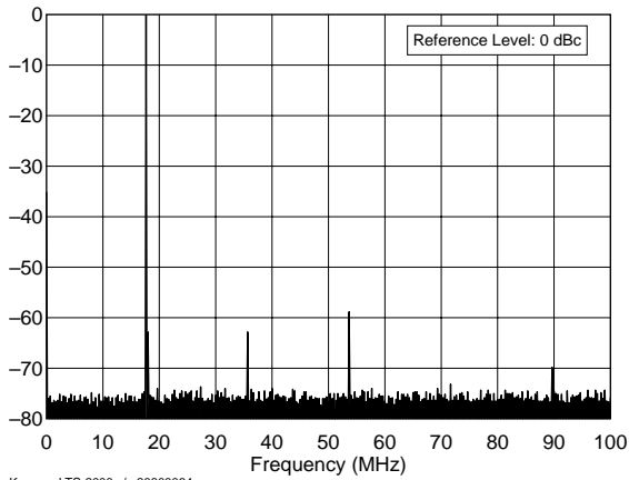
Kenwood TS-2000 s/n 20800064 18.1 MHz Band, Spectral Purity, 100 W F:\SHARED\PROD_REV\TESTS\TS2000\TS200S17.TXT
