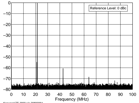
Kenwood TS-2000 s/n 20800064 21.0 MHz Band, Spectral Purity, 100 W F:\SHARED\PROD_REV\TESTS\TS2000\TS200S15.TXT
