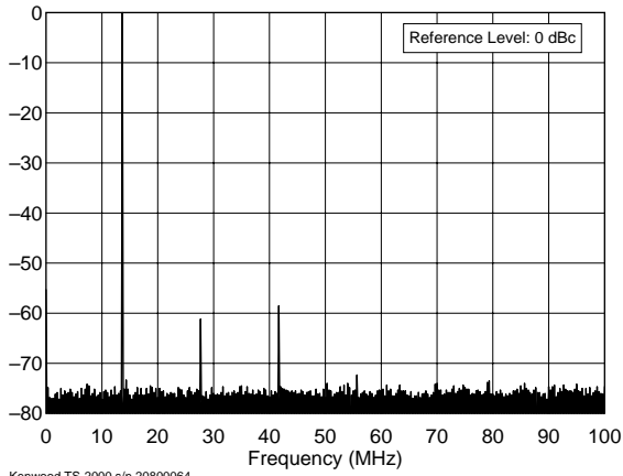
Kenwood TS-2000 s/n 20800064 14.0 MHz Band, Spectral Purity, 100 W F:\SHARED\PROD_REV\TESTS\TS2000\TS200S20.TXT
